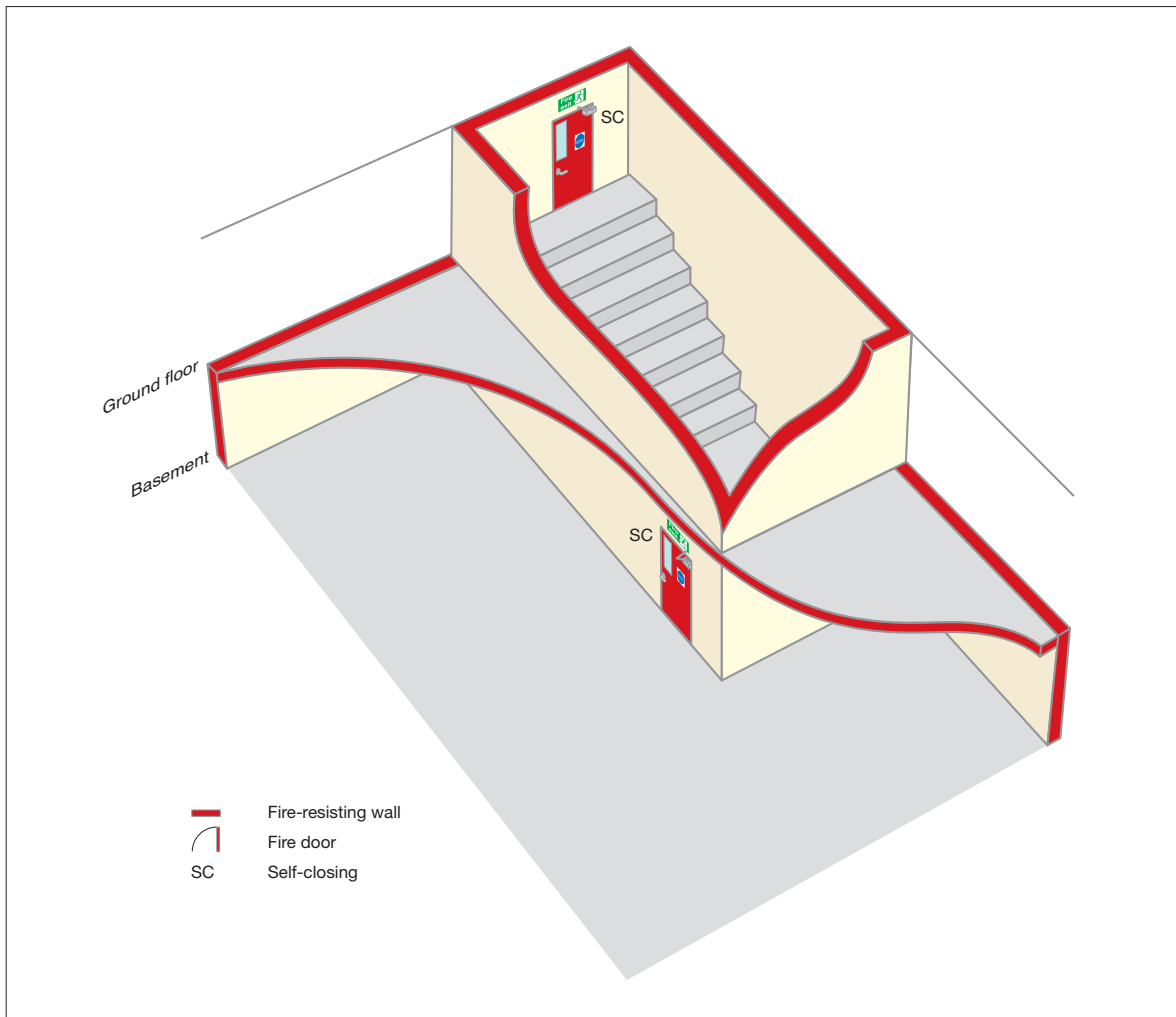
Figure 39: Basement protection
