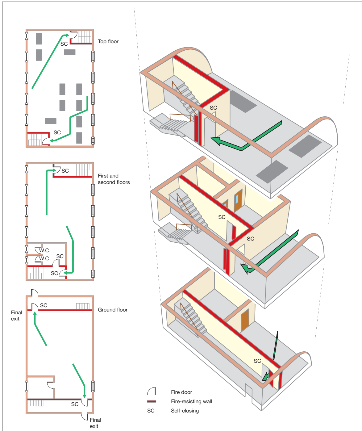
Figure 54: Four-storey premises: ground and up to three upper floors
